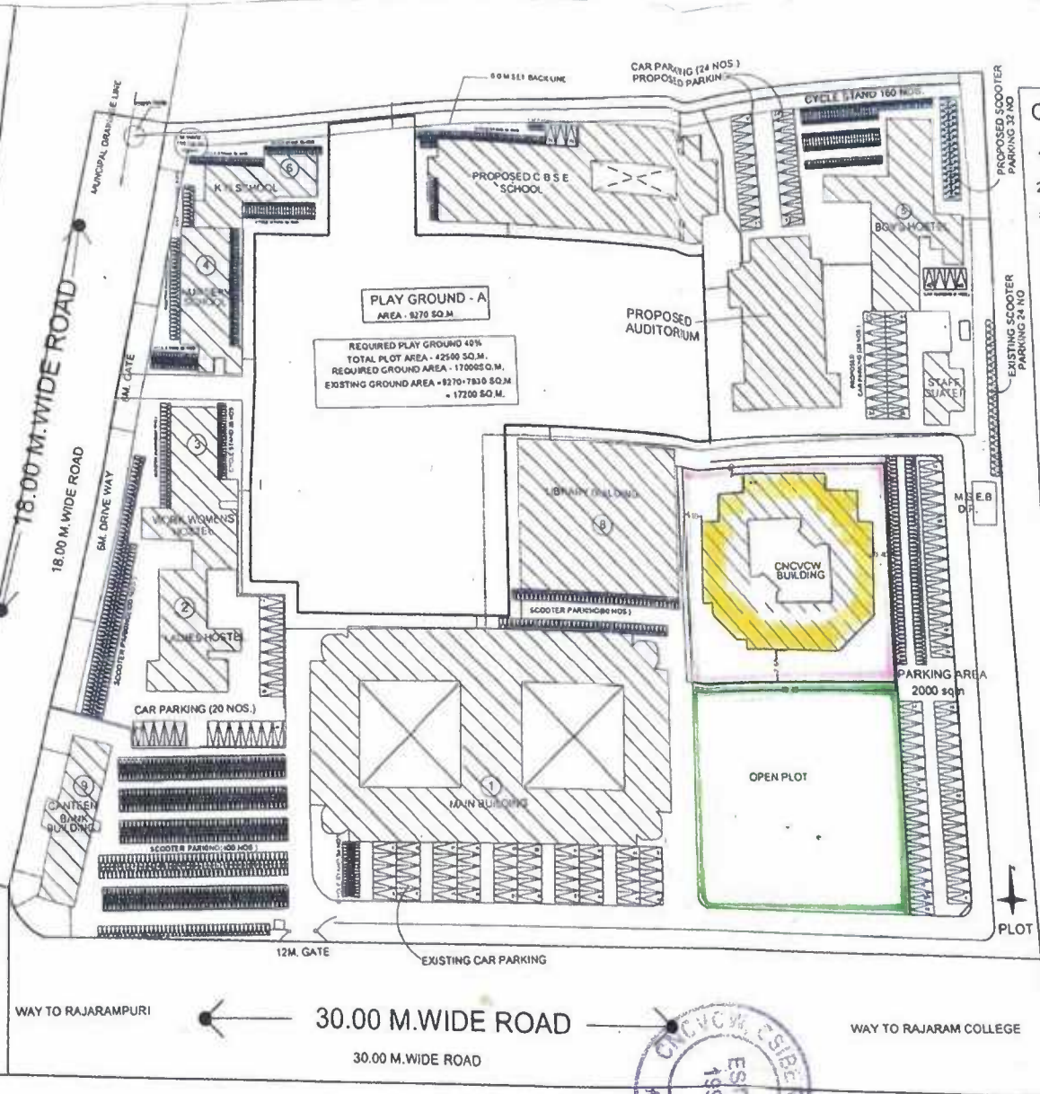
CSIBER CAMPUS SITE PLAN WITH AREA STATEMENT FOR CNCVCW
